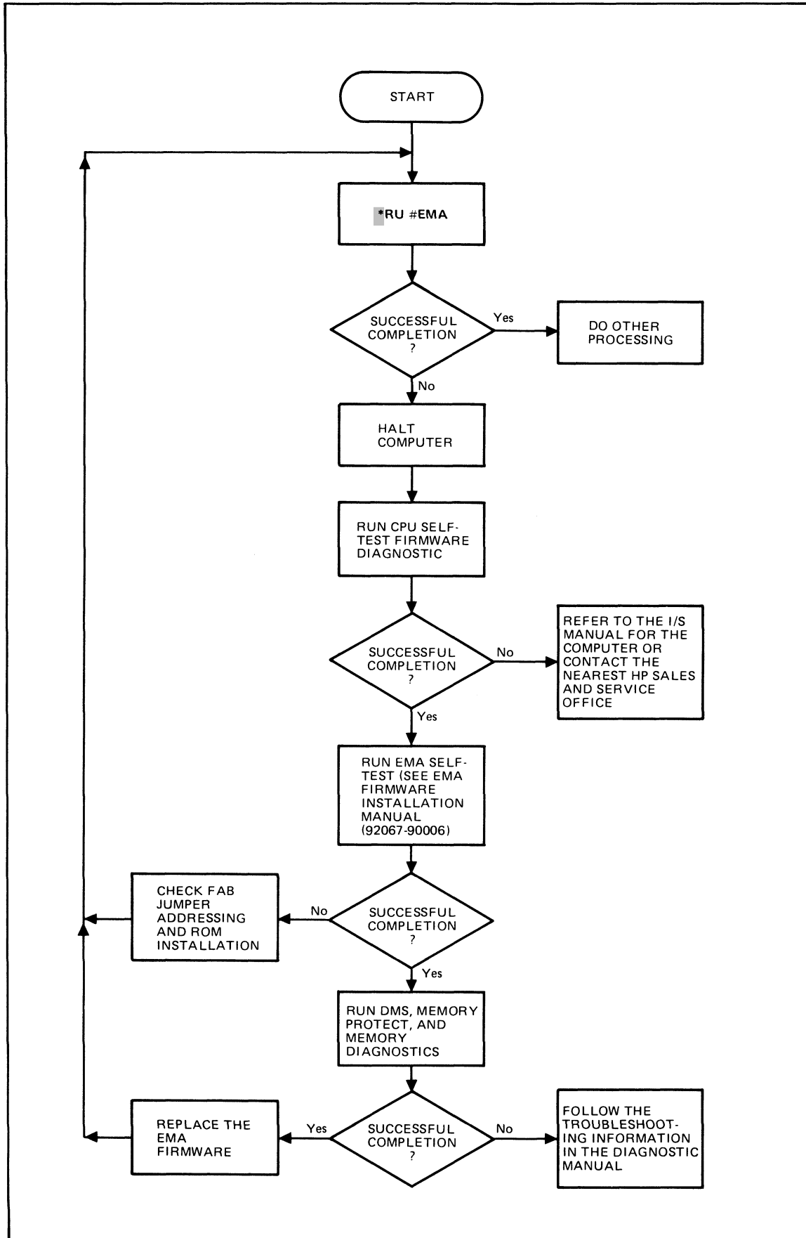
Figure 4-1. Troubleshooting Flowchart
